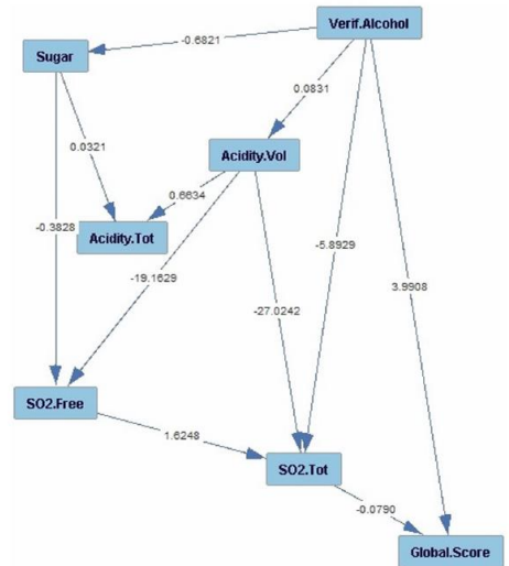
Fig. 3. Red and white wines. The causal DAG with the estimates of the linear SEM parameters as edge weights for the chemical variables and the GSO.
